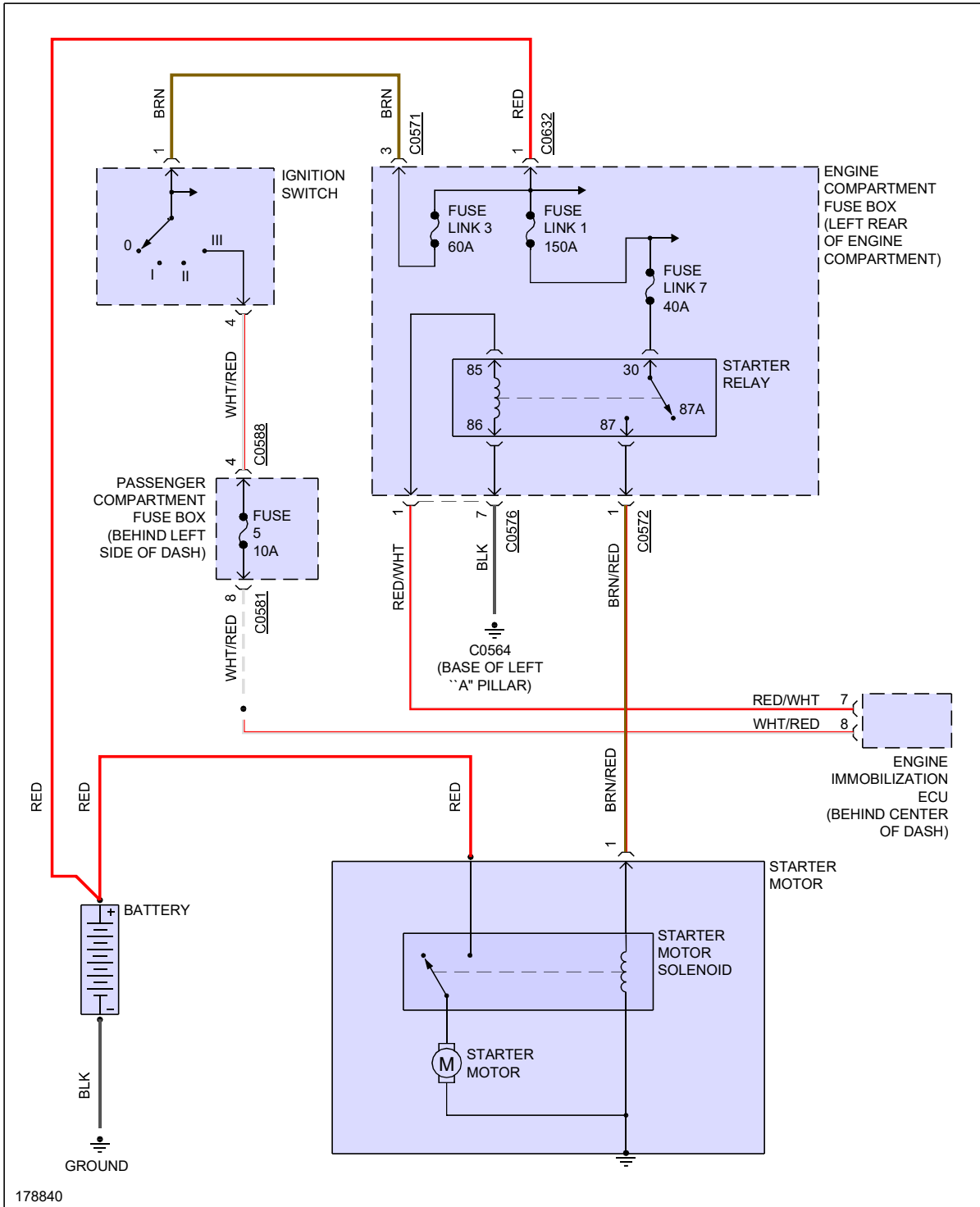
Fig 2: Starting Circuit
