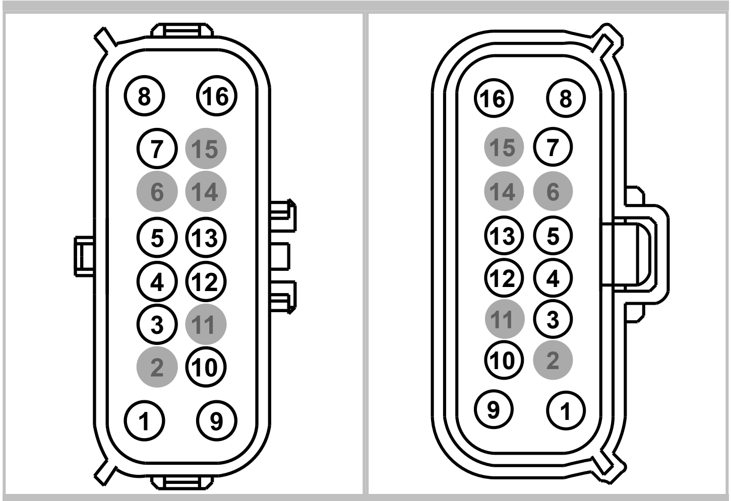
MALE Harness 14405
