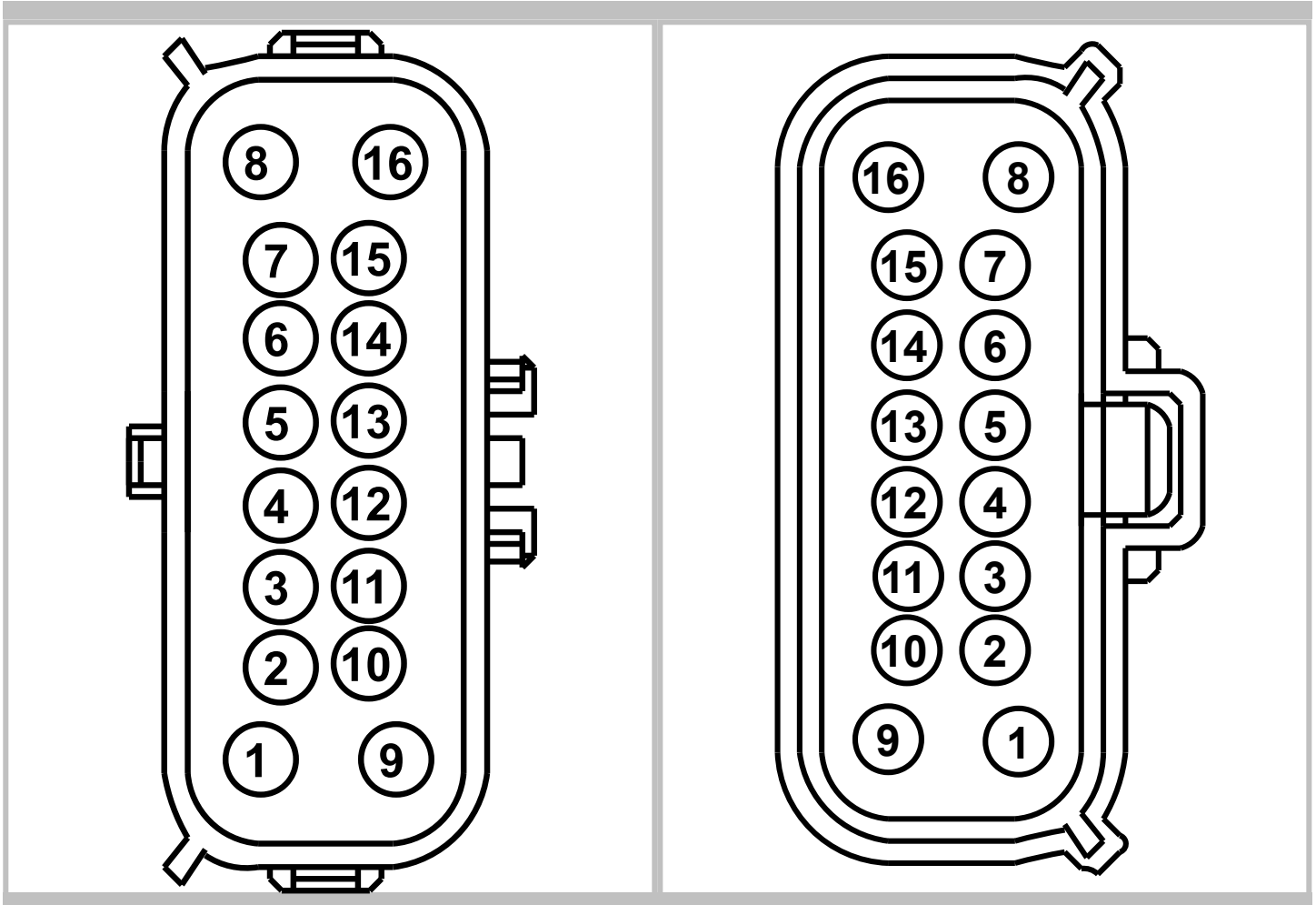
MALE Harness 12A581
