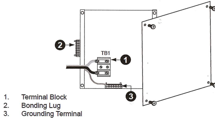
Figure B Control Box
