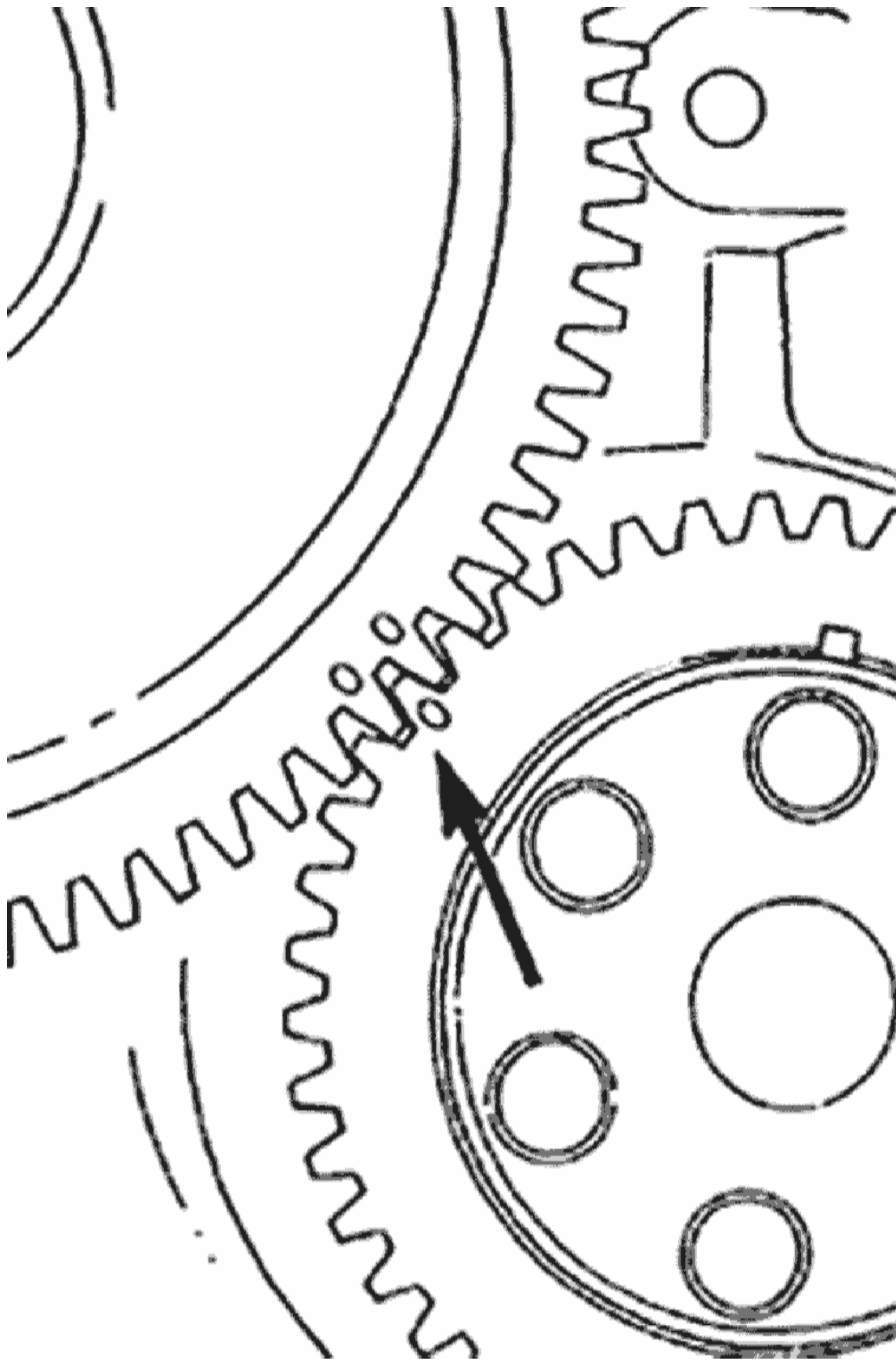
Camshaft & accessory drive gear timing marks
