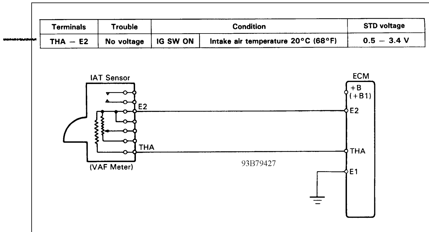
Fig 1: DTC 24 - Schematic
