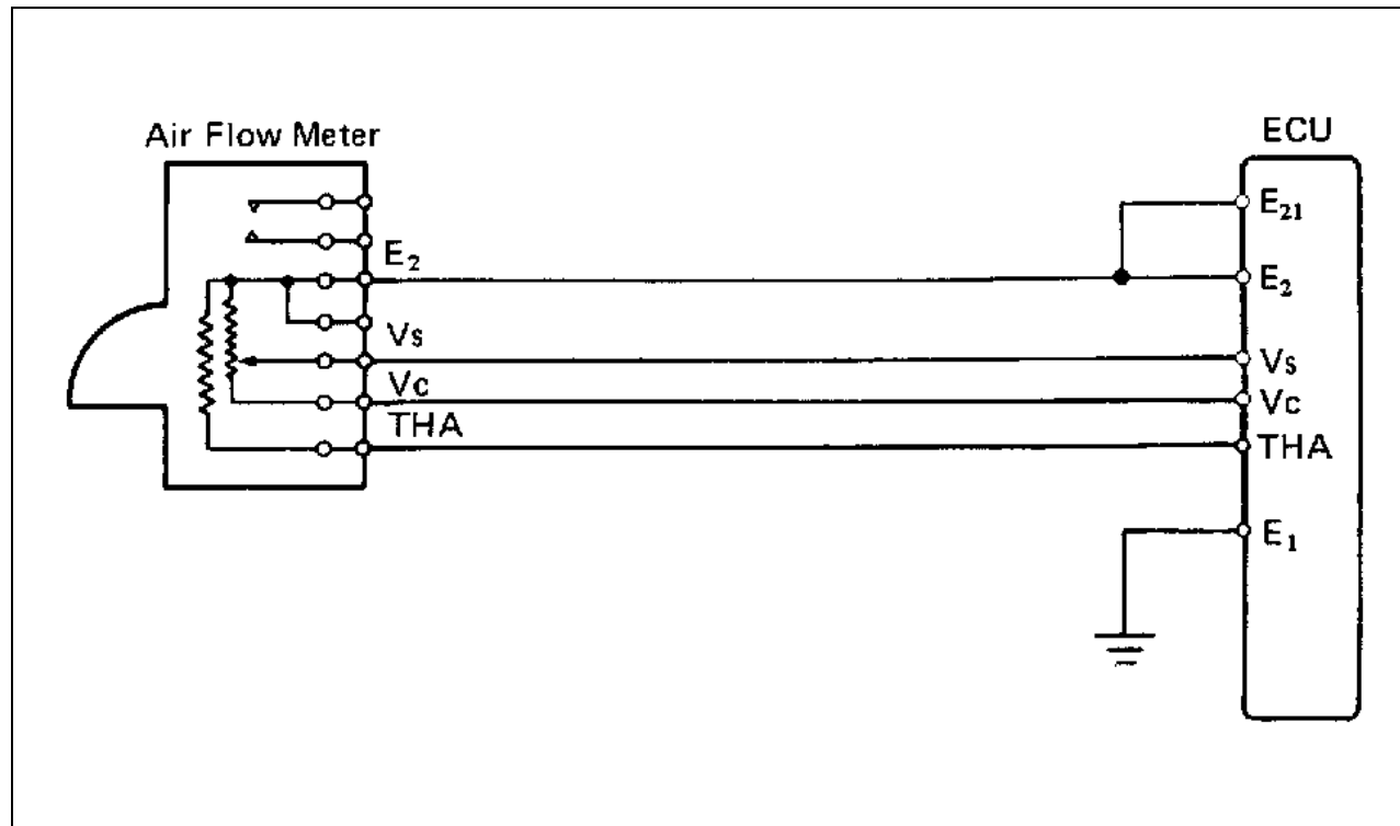
Fig 1: Code 24, 31, 32/Test No. 5 Schematic Intake Air Temp. Sensor & Airflow Meter Signal
