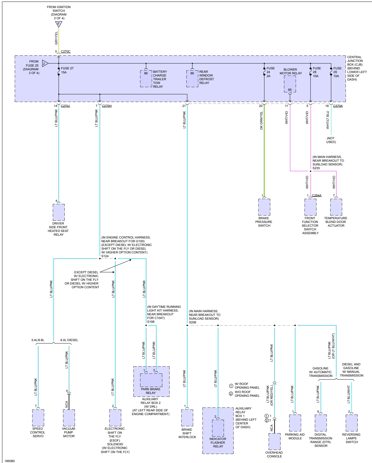
Fig 4: Power Distribution Circuit (4 of 4)
