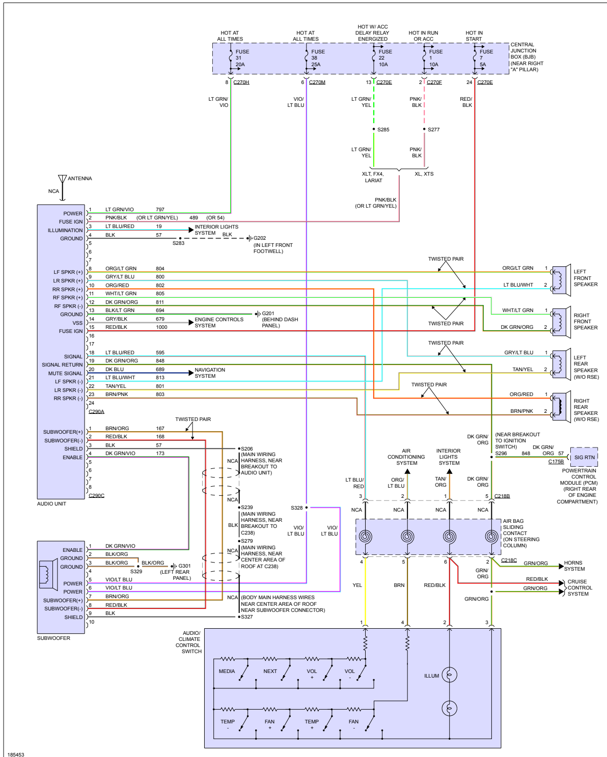
Fig 2: Radio Circuit, Premium Radio
