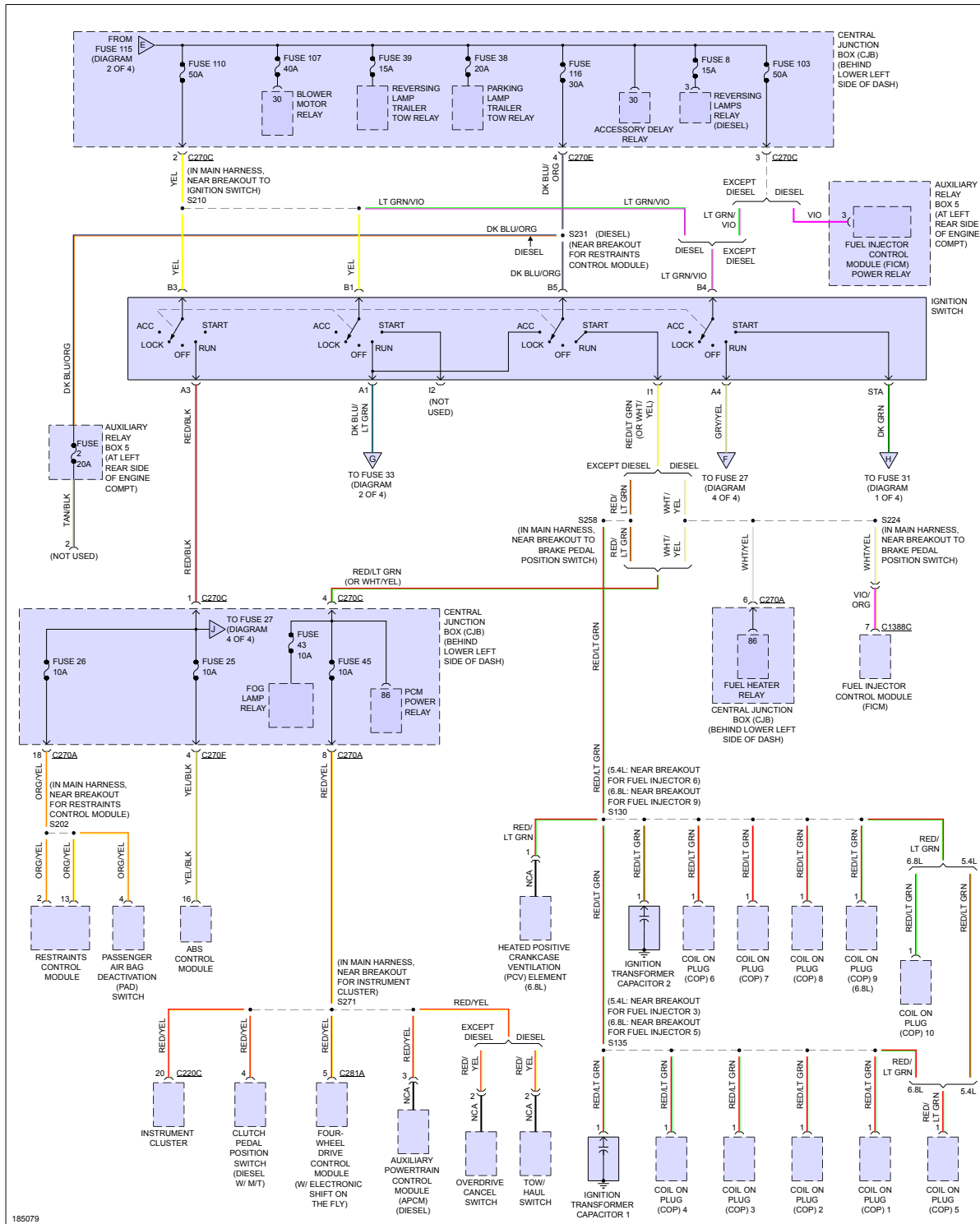
Fig 3: Power Distribution Circuit (3 of 4)
