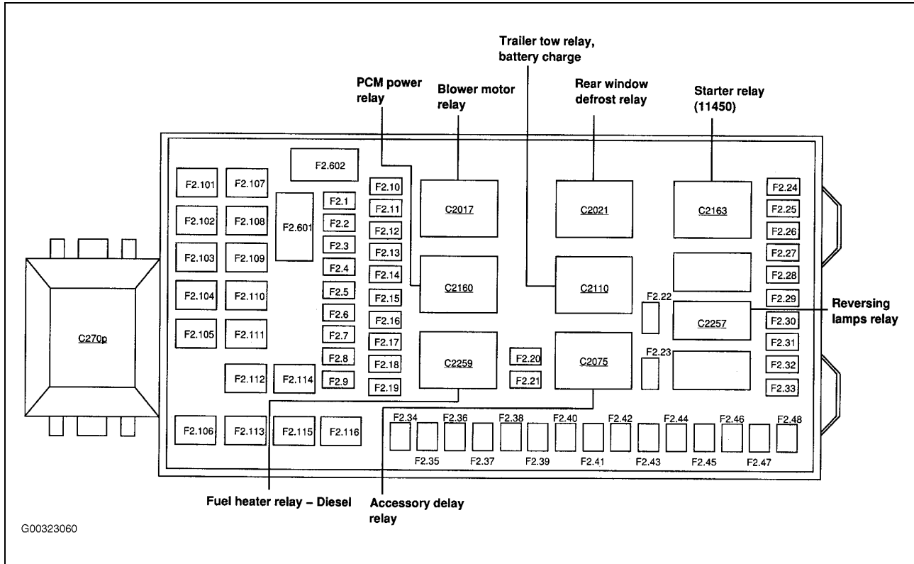
Fig 2: Central Junction Box Components, Fuses And Relays
