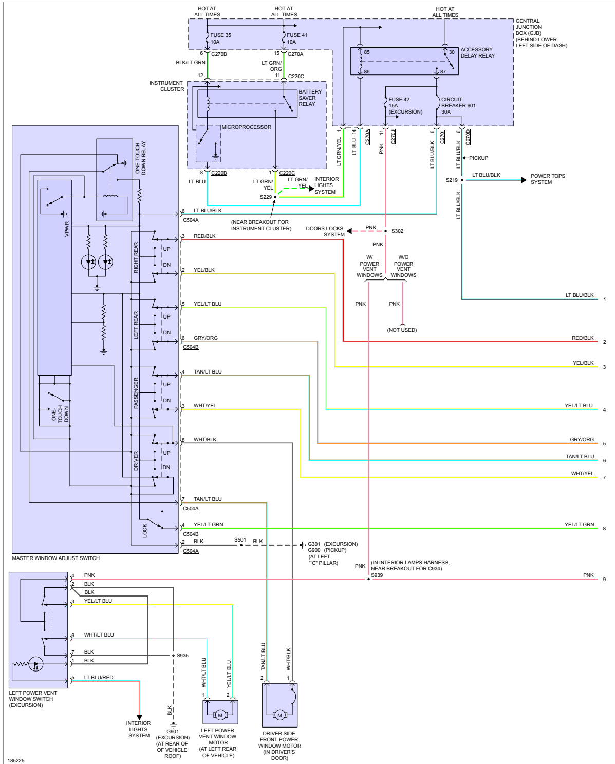
Fig 1: Power Windows Circuit, Crew Cab (1 of 2)
