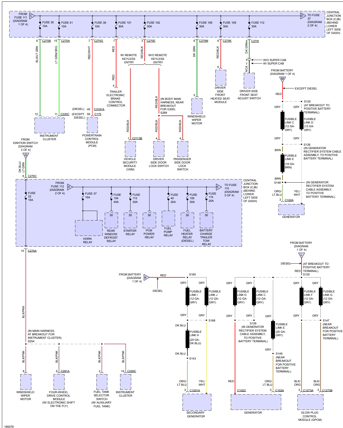
Fig 2: Power Distribution Circuit (2 of 4)
