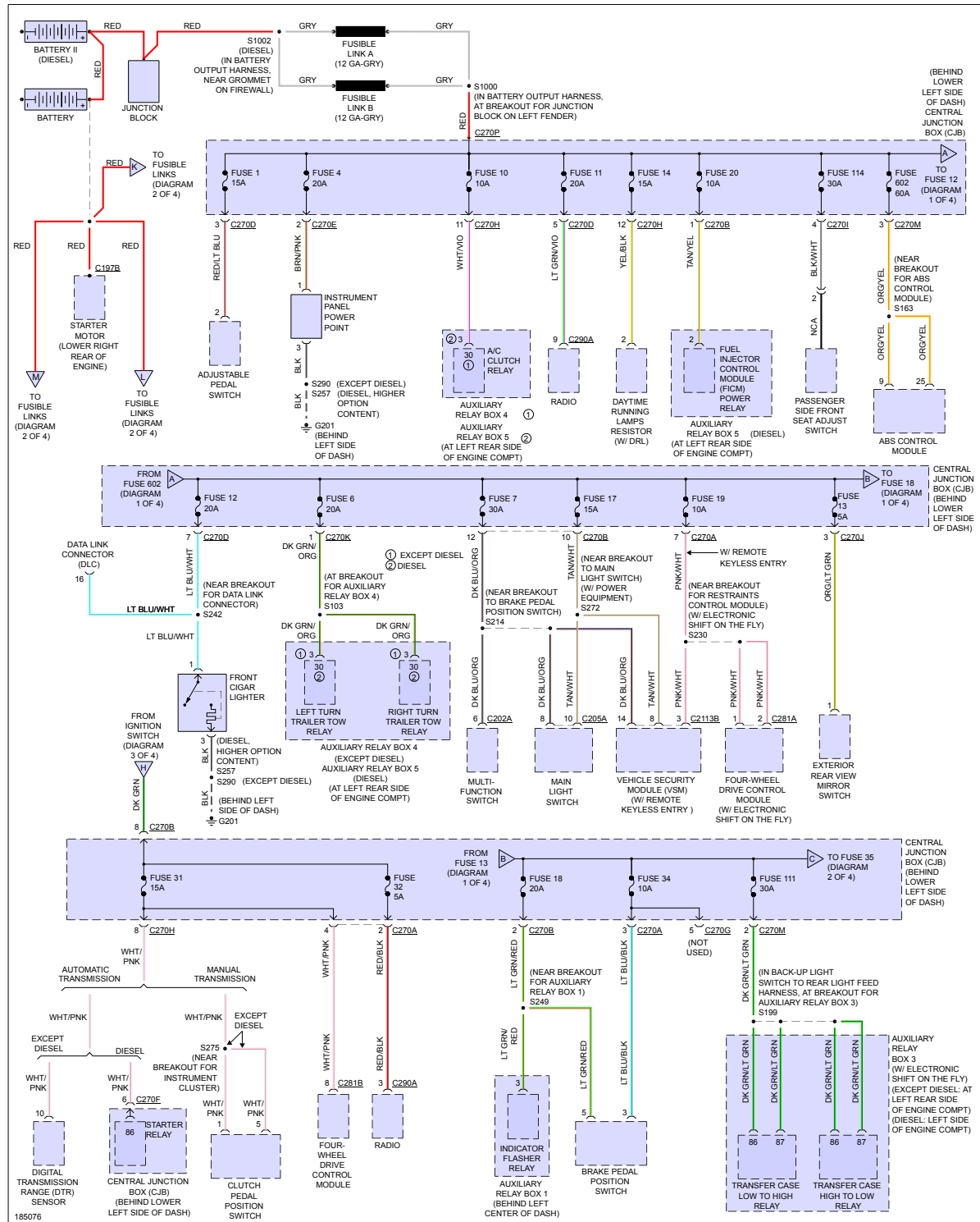
Fig 1: Power Distribution Circuit (1 of 4)
