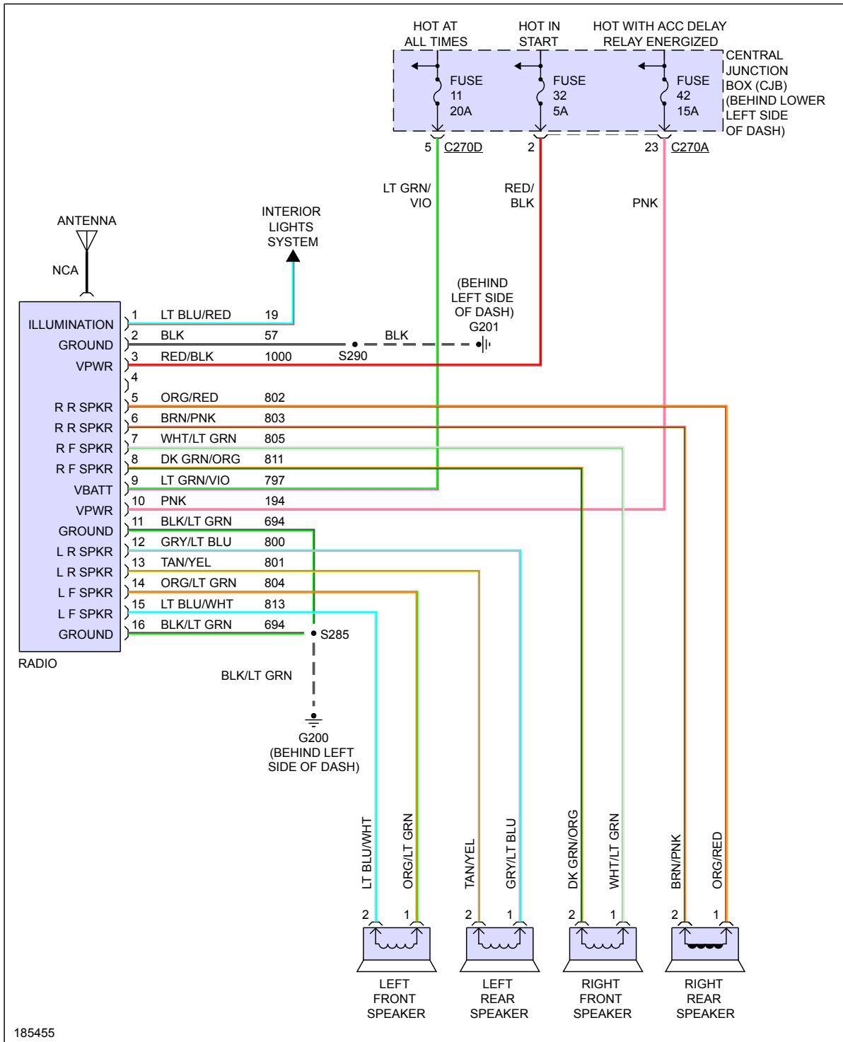
Fig 1: Radio Circuit
