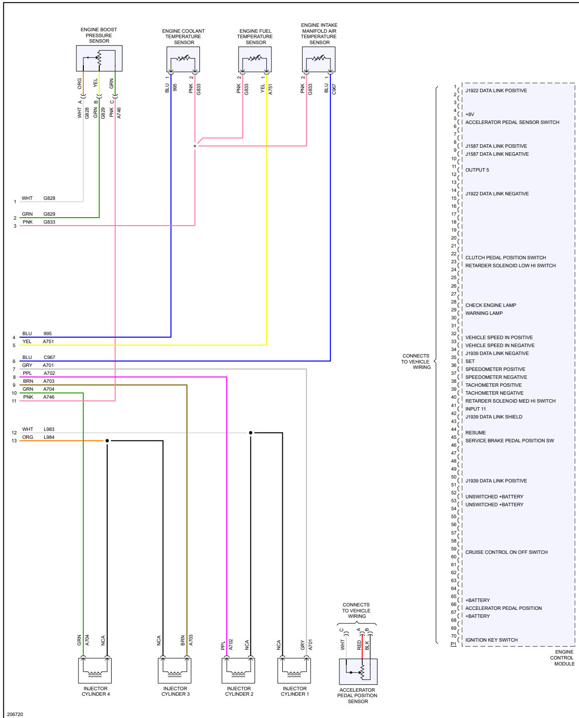
Fig 2: Caterpillar Engine Performance Wiring Diagram (C-15 - 6N21 - 2 Of 2)
