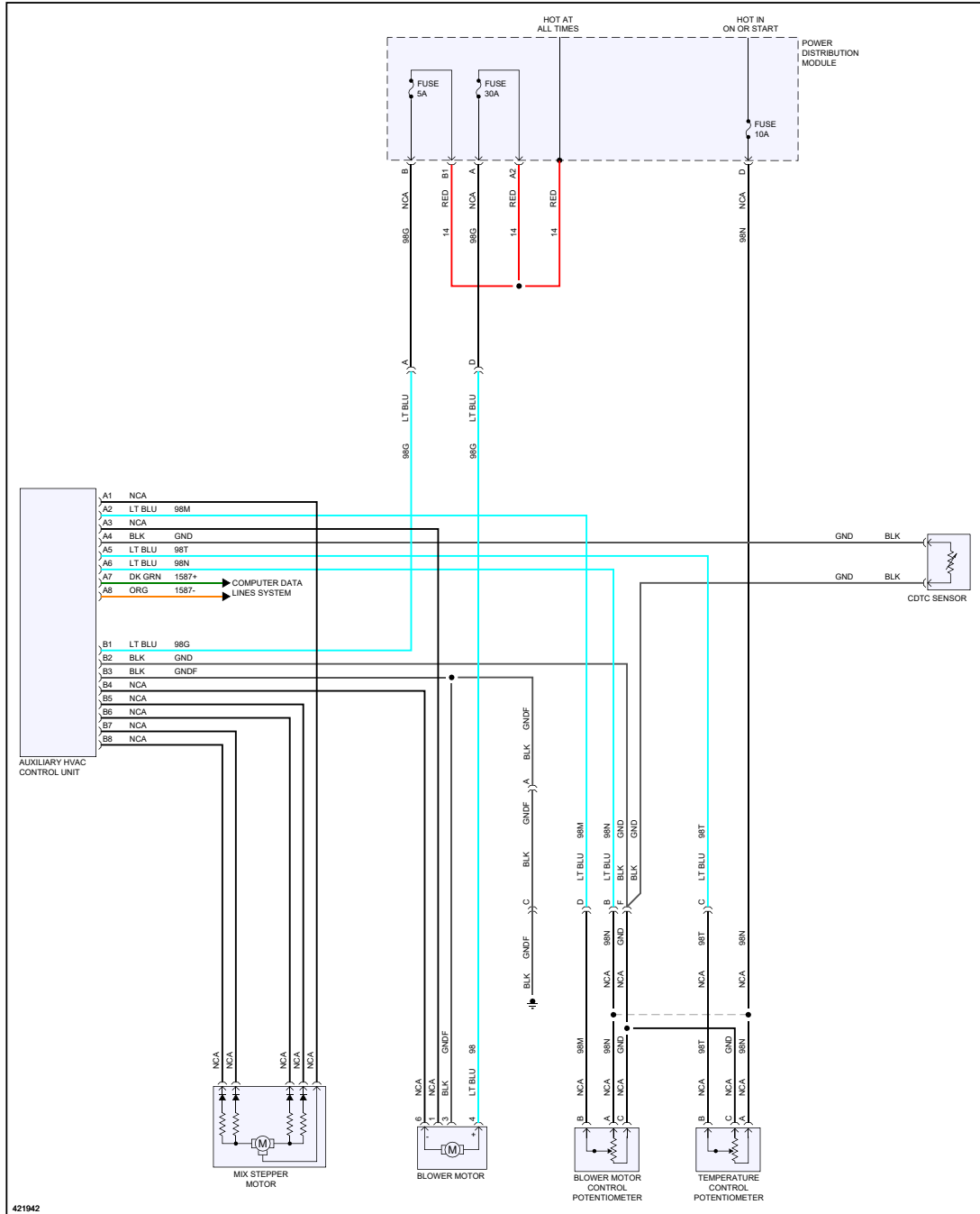
Fig 1: Auxiliary A/C Circuit
